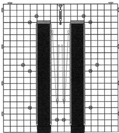
UNIVERSAL Float-Plane AquaPad™ Distance between floats (on-center): 70" - 130" Size: 28'4" wide x 35' long Cubes: 353 Item No.: T.B.D
